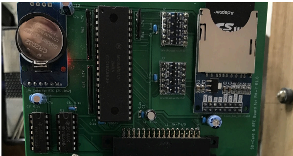
RTC-SD card
